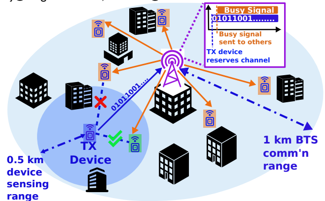
Figure 1: The sensing channels are significantly inferior to communication channels in urban wide-area deployments. BSMA alleviates the hidden node problem by transmitting a Busy Signal during ongoing uplink transmissions.
