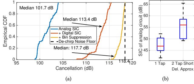
Figure 13: (a) CDF of BSMA's SIC over 10 seconds, split into component stages. Analog SIC provides a median cancellation > 100 dB. Digital cancellation provides additional 12 dB, and finally, bin suppression takes SI to the instrument noise floor. We measure median noise floor degradation of 0.7 dB in the de-chirped domain since the residual SI leaks to some adjacent bins. (b) Analog cancellation performance across 7 locations using a single tap vs our two tap (short delay approximation). Only our two tap approach consistently meets the cancellation budget.
