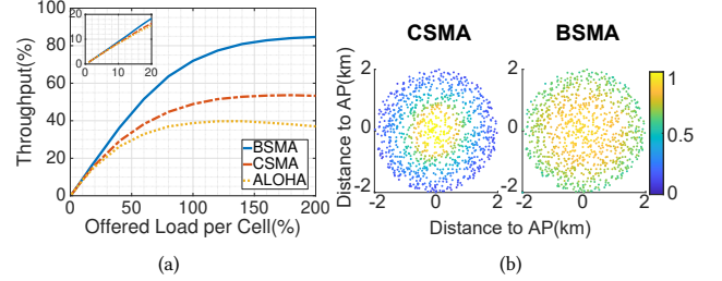
Figure 12: Thousand device simulations: (a) throughput performance (b) PRR distribution w.r.t device location. Each dot is a device, and its PRR is encoded in the color (brighter the better). BSMA therefore improves throughput while maintaining fairness.
