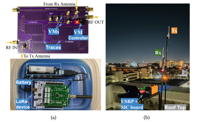
Figure 9: Elements of the Testbed. (a) Top: The Full Duplex PCB featuring short-delay traces and vector modulators. Bottom: A battery-powered LoRa device in a box enclosure. (b) Rooftop gateway deployment. We deploy the devices outdoor on the university campus.
